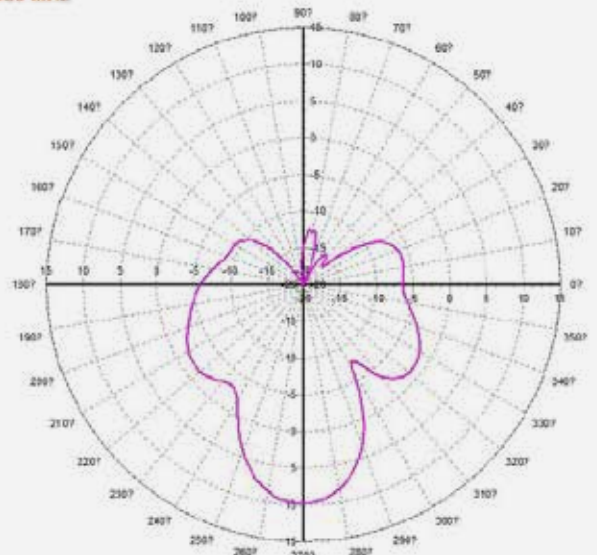
2.4G (PHI=90)
