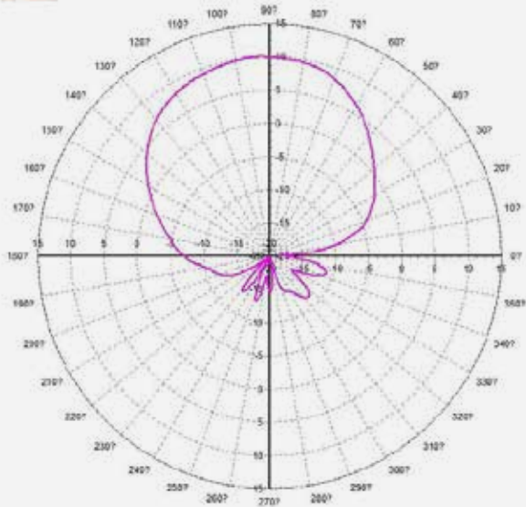
2.4G (PHI=0)
