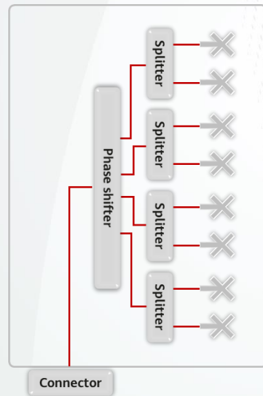
Figure: Energy route inside antennas
